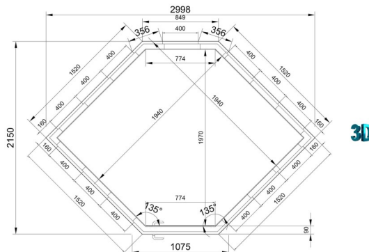
Studio - Plus - D - Multi - Angle = 16400,00 € Int. 3.5 m 2 Ext. 4.1 m 2 - 1117 kg.
