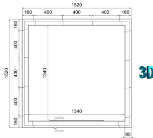
Studio - Plus - II = 1030,00 € Int. 1.8 m2 Ext. 2.3 m2 - 786 kg.
