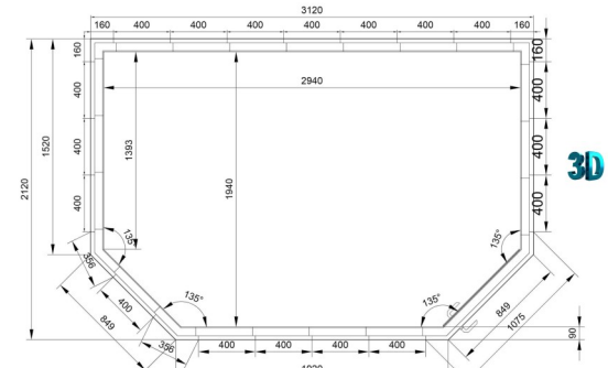
Studio - Plus - F - Multi - Angle = 21300,00 € Int. 5.6 m 2 Ext. 6.4 m 2 - 1472 kg.
