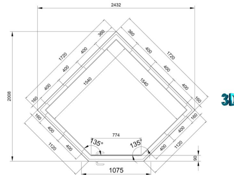
Studio - Plus - B - Multi - Angle = 11920,00 € Int. 2.3 m 2 Ext. 2.8 m 2 - 853 kg.
