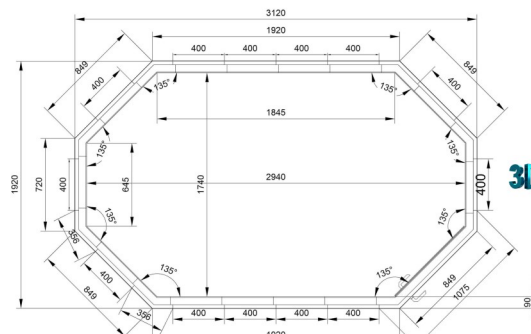
Studio - Plus - E - Multi - Angle = 24850,00 € Int. 5.5 m 2 Ext. 6.3 m 2 - 1458 kg.
