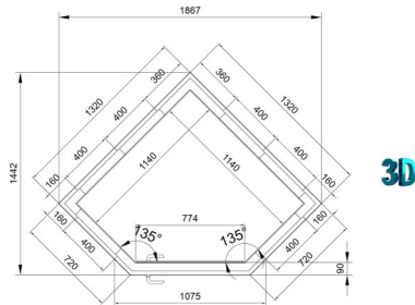
Studio - Plus - A - Multi - Angle = 7860,00 € Int. 1.2 m 2 Ext. 1.6 m 2 - 589 kg.
